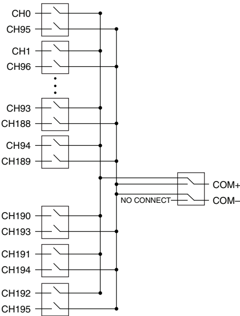
Figure 1. NI 2575 Hardware Diagram
